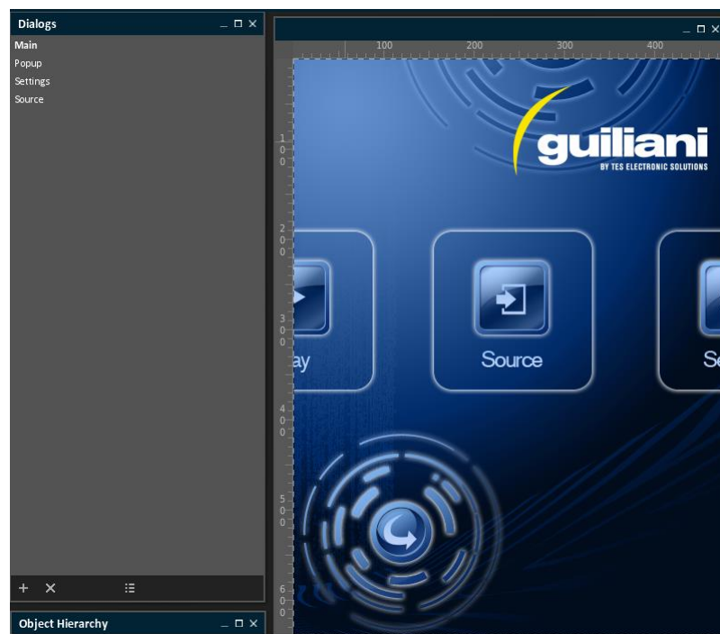
Fig. 1 Editor Demo
