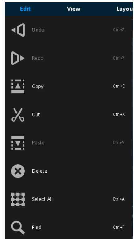
Fig 18 - Edit Menu
