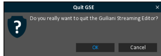
Fig 16 - Quit
