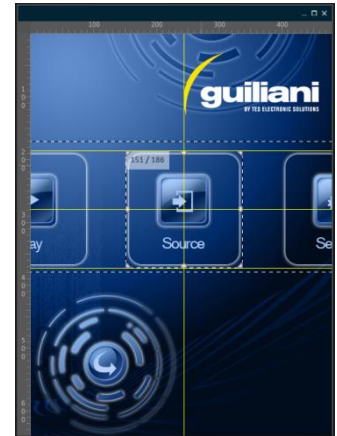
Fig 47 - Assisting Guidelines
