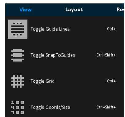
Fig 20 - View Menu
