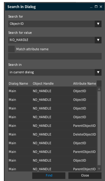
Fig 19 - Find
