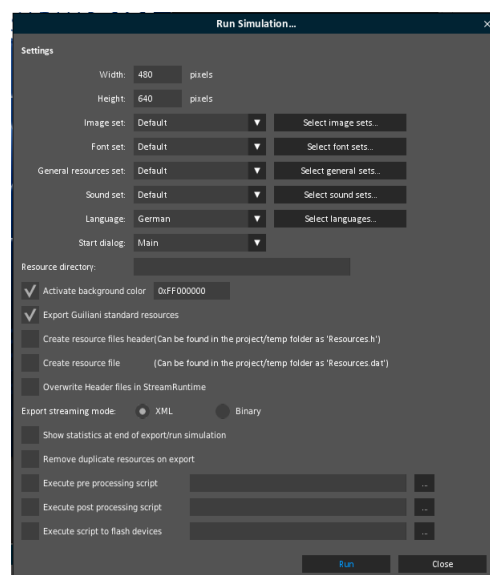
Fig 15 - Run Simulation window
