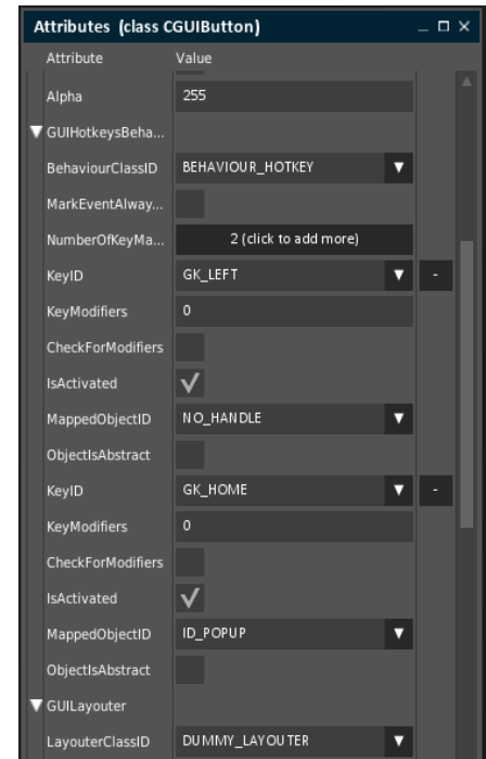
Fig 49 - GUI Hotkey Behaviour
