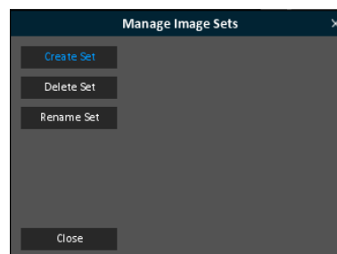
Fig 33 - Manage Sets
