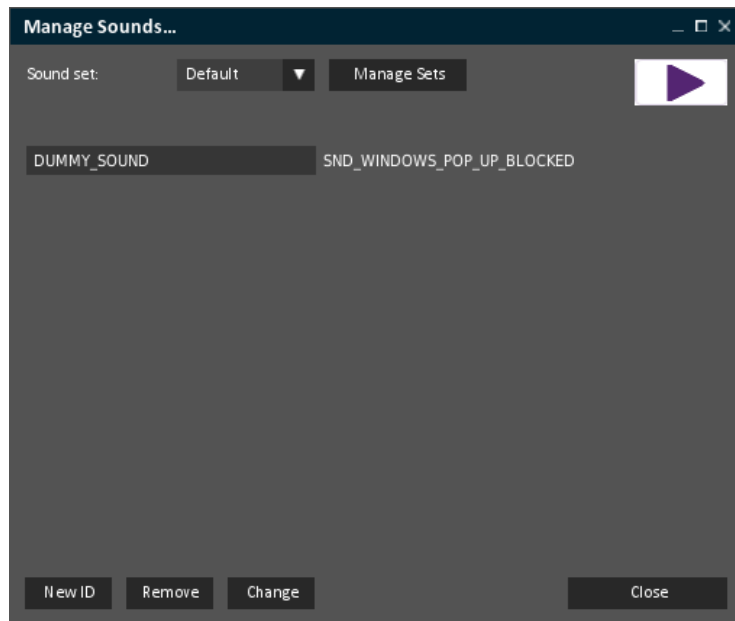
Fig 31 - Manage Sounds
