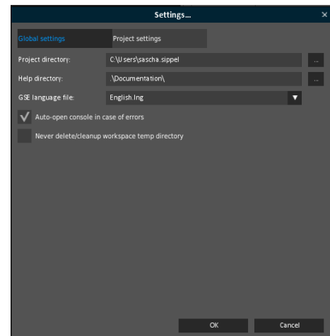
Fig 10 - Global Settings
