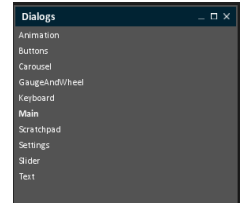
Fig 45 - Workspace Window
