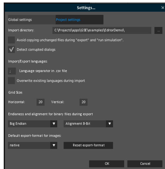
Fig 11 - Project Settings
