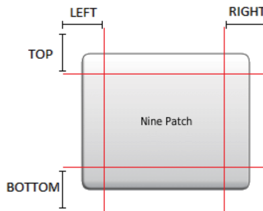
Fig 2 - Nine Patch
