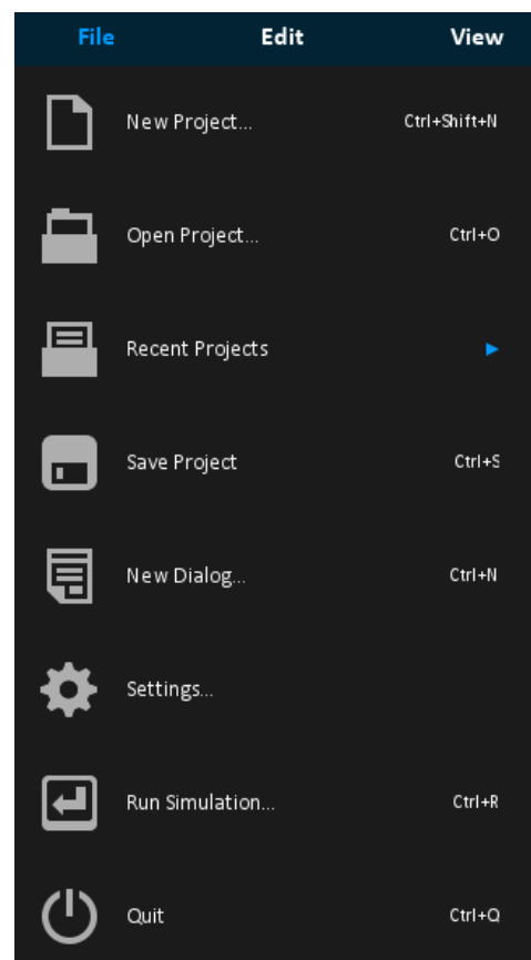
Fig 4 - File Menu
