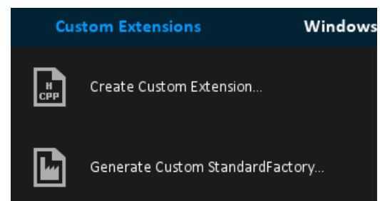
Fig 41 - Custom Extension
