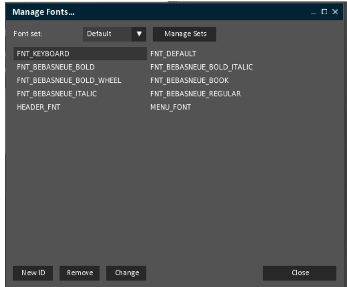
Fig 29 - Manage Fonts
